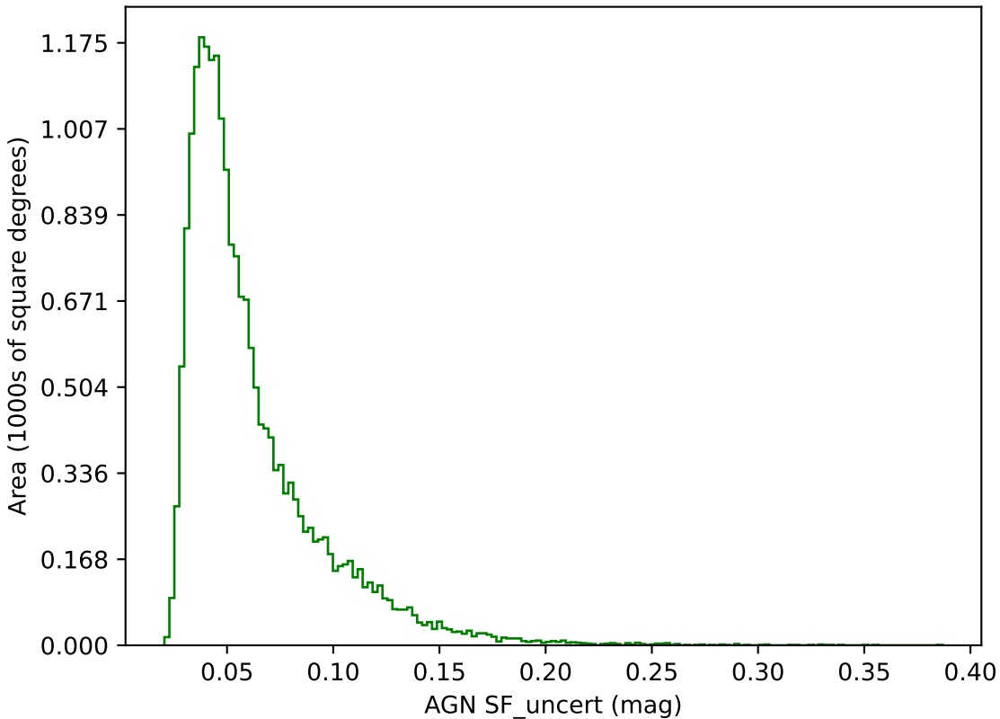
too_elab_r128_d3_giz_v3.4_10yrs g band: AGN SF_uncert
