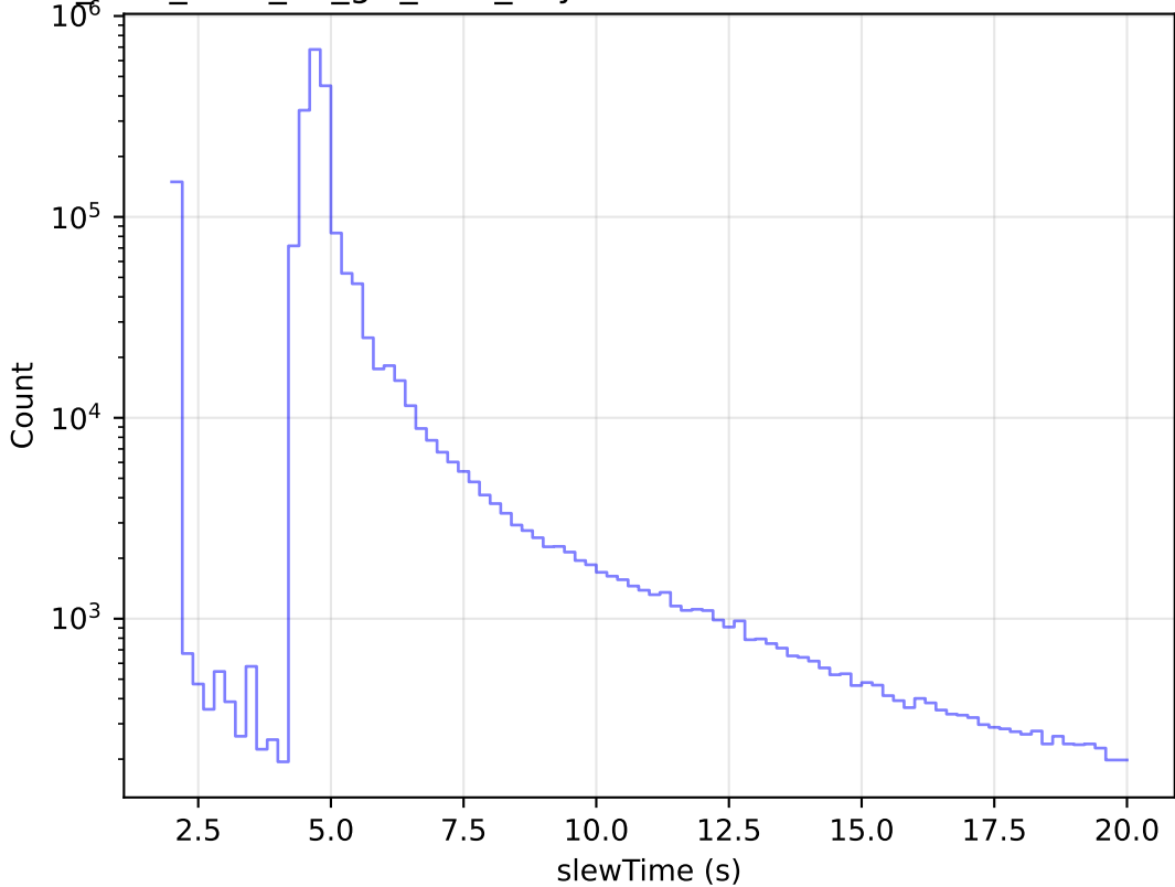
too_elab_r128_d3_giz_v3.4_10yrs All visits: Zoom Slew Time Histogram
