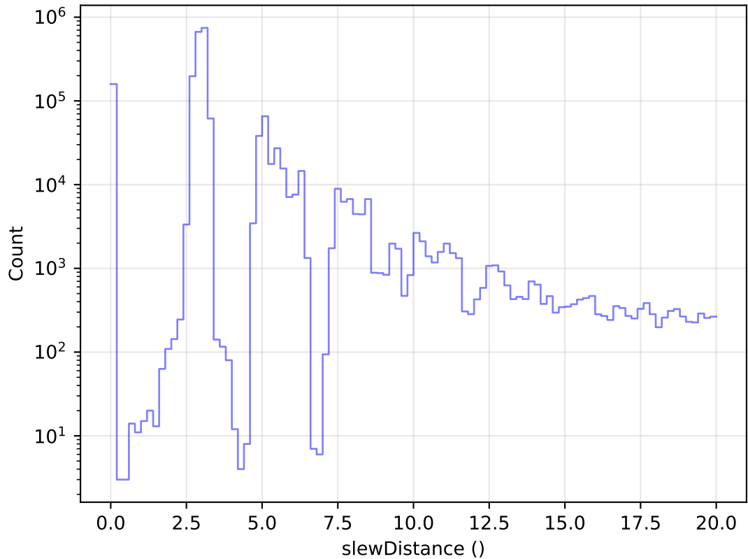
too_elab_r128_d3_giz_v3.4_10yrs All visits: Zoom Slew Distance Histogram
