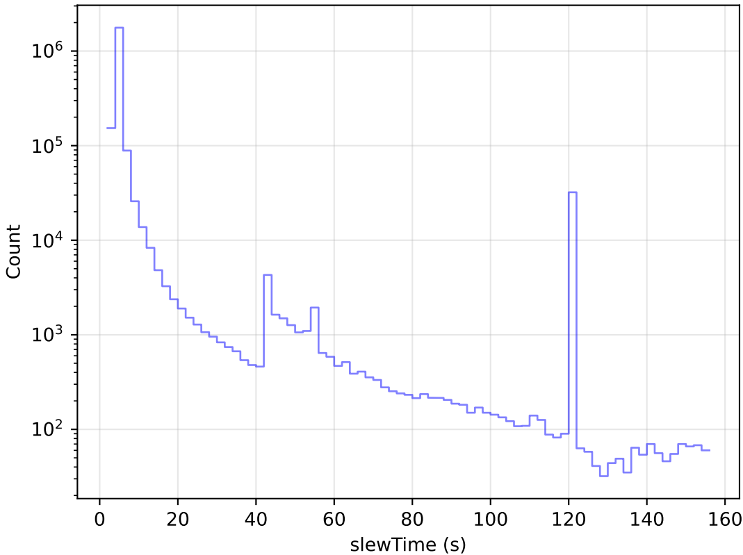
too_elab_r128_d3_giz_v3.4_10yrs All visits: Slew Time Histogram
