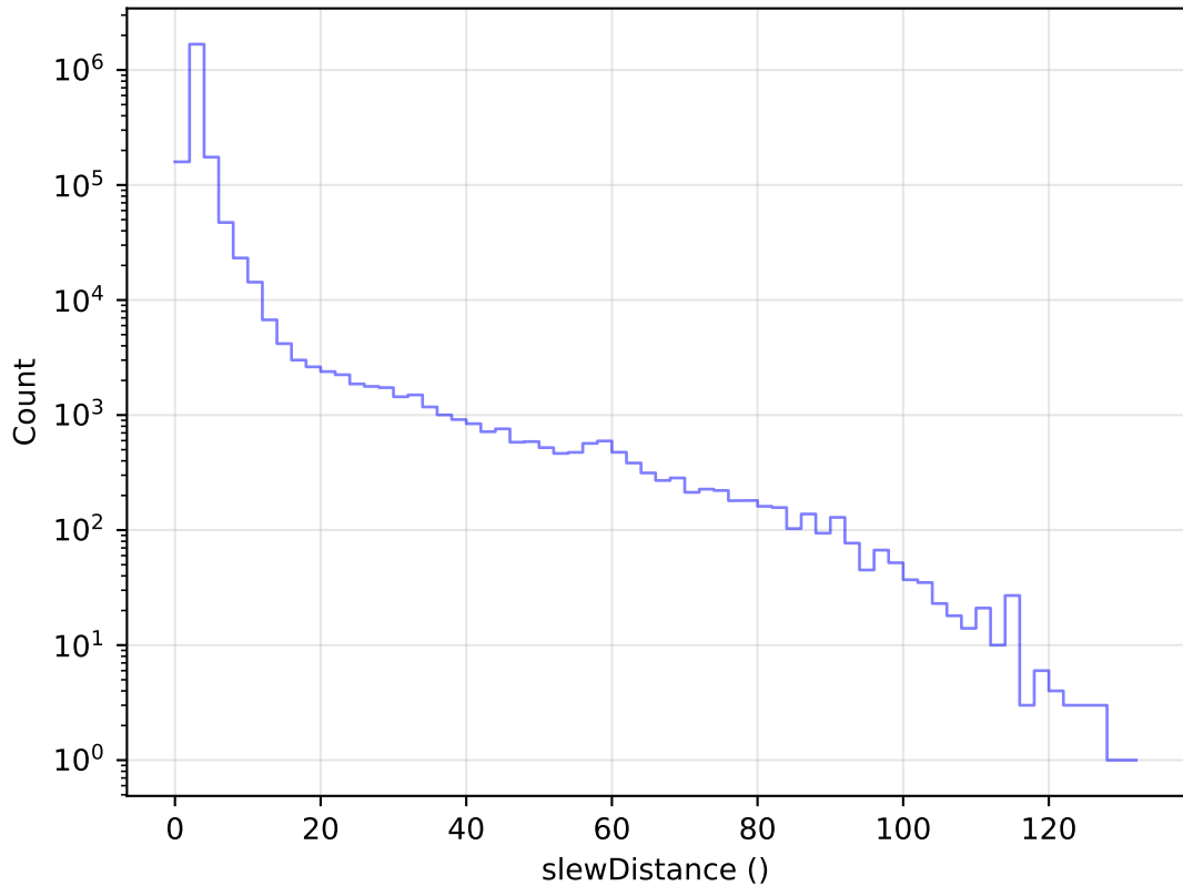
too_elab_r128_d3_giz_v3.4_10yrs All visits: Slew Distance Histogram
