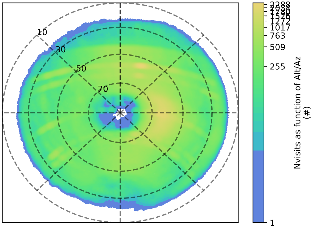
too_elab_r128_d3_giz_v3.4_10yrs z: Nvisits as function of Alt/Az
