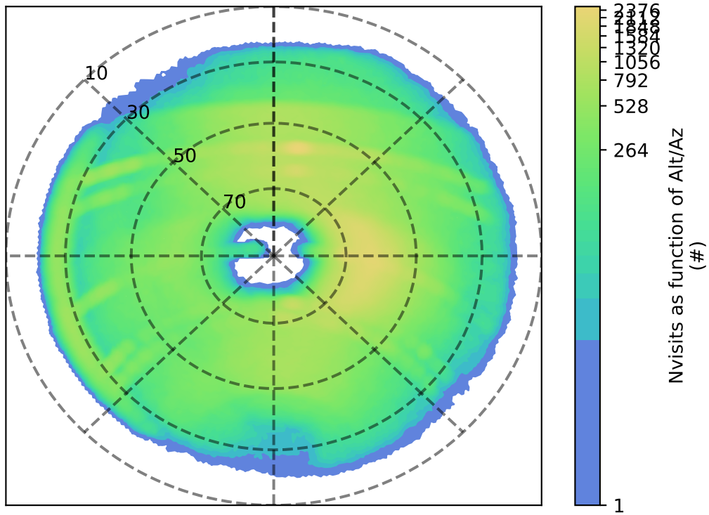
too_elab_r128_d3_giz_v3.4_10yrs r: Nvisits as function of Alt/Az
