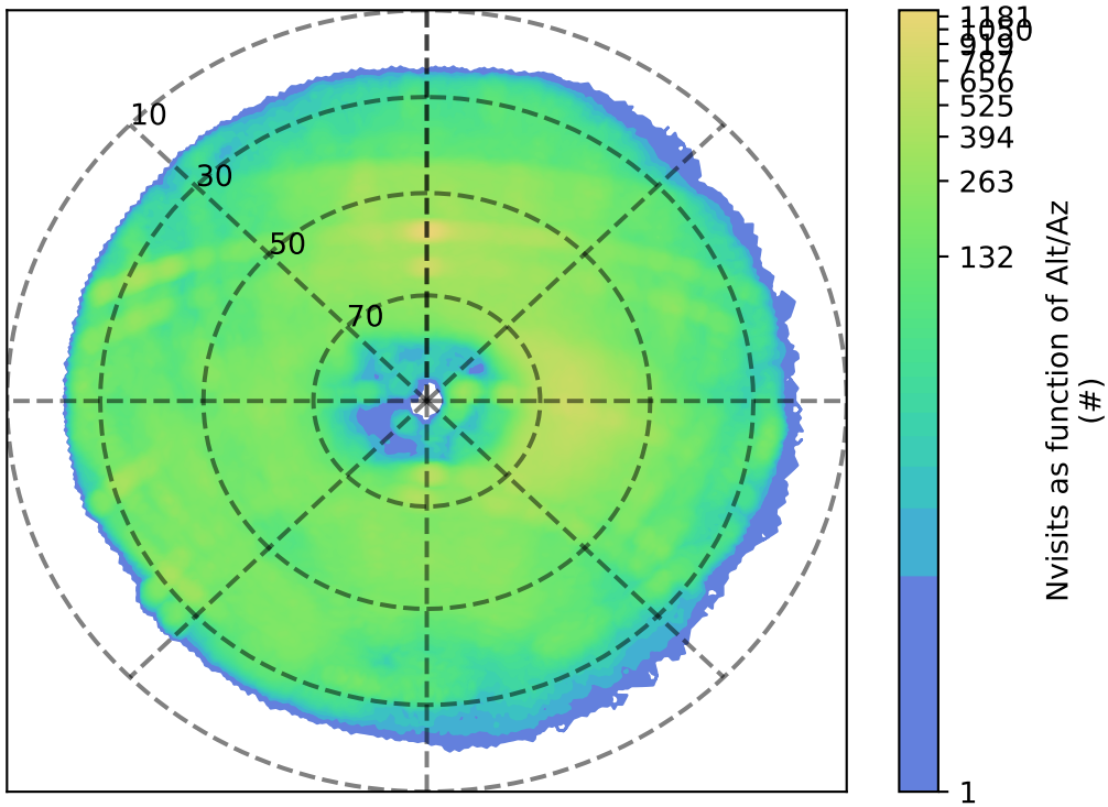
too_elab_r128_d3_giz_v3.4_10yrs g: Nvisits as function of Alt/Az
