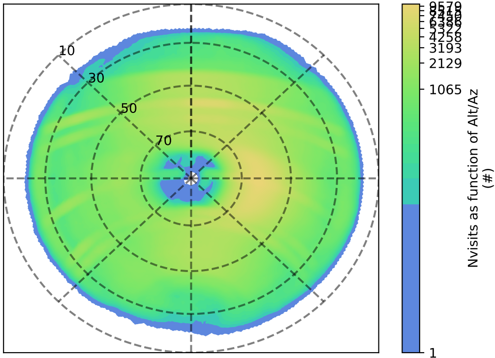
too_elab_r128_d3_giz_v3.4_10yrs : Nvisits as function of Alt/Az
