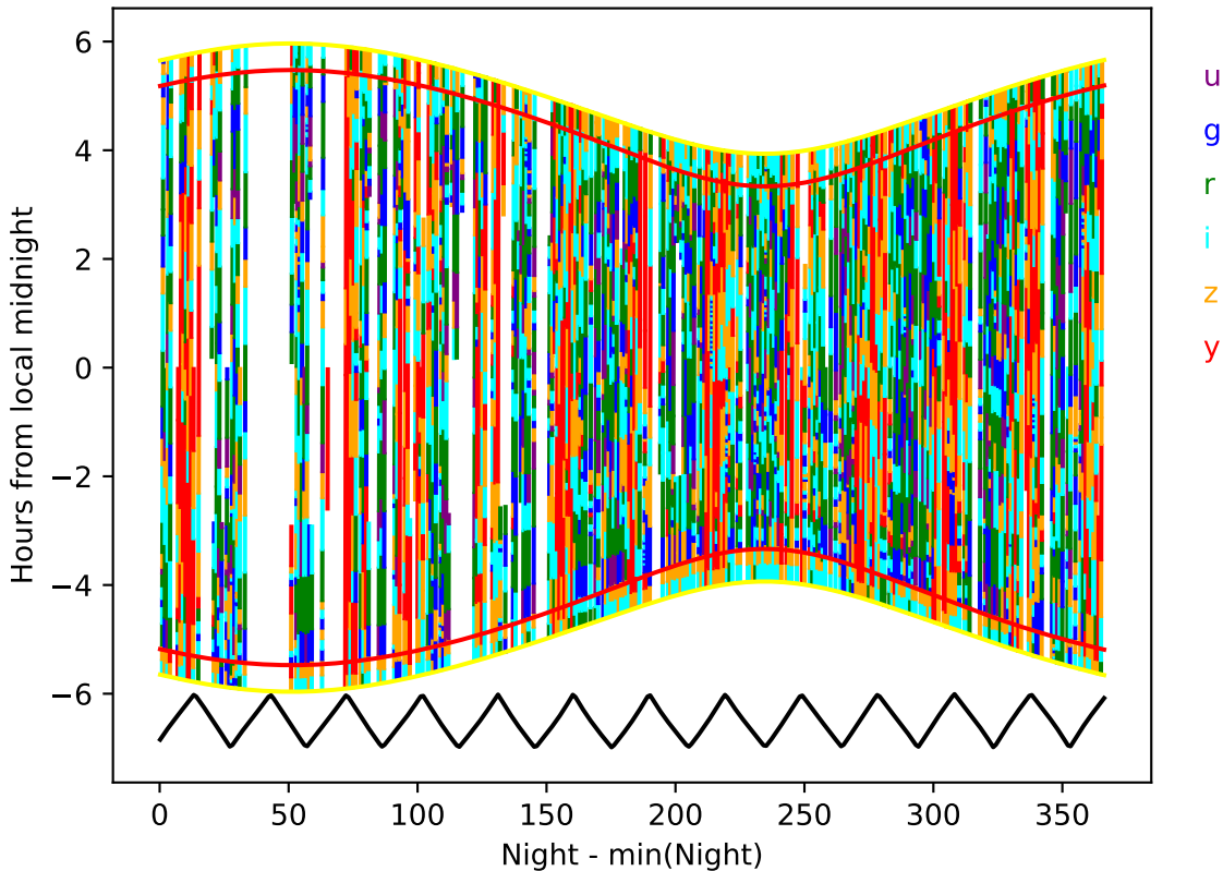
too_elab_r128_d3_giz_v3.4_10yrs year 8-9: Hourglass
