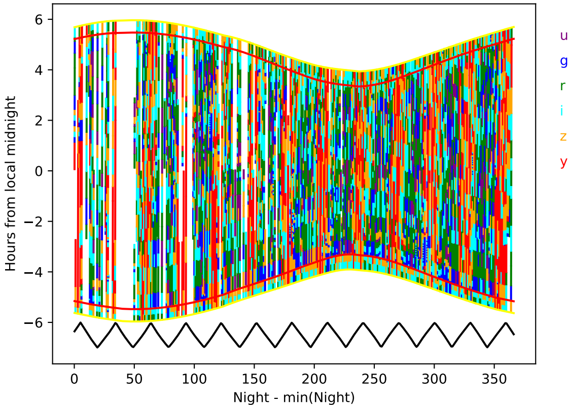
too_elab_r128_d3_giz_v3.4_10yrs year 6-7: Hourglass
