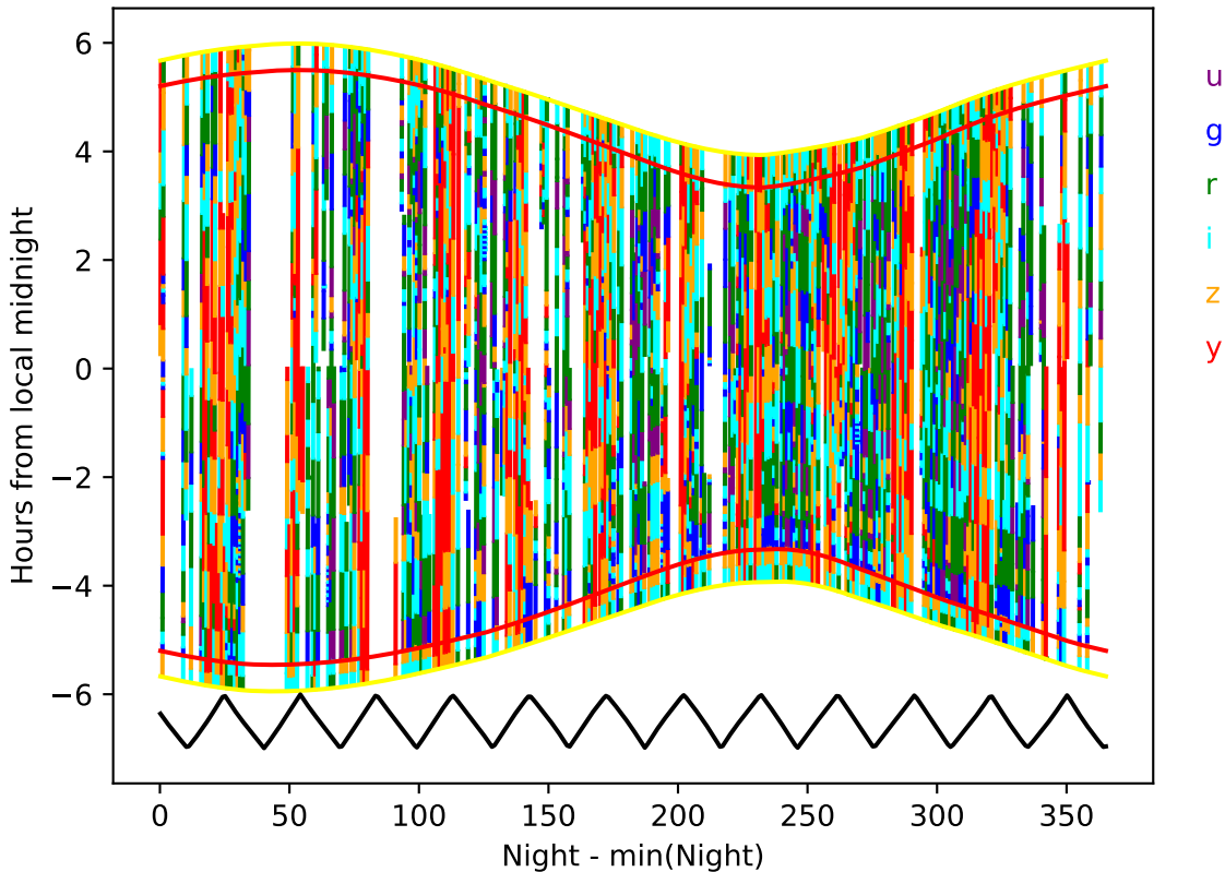
too_elab_r128_d3_giz_v3.4_10yrs year 4-5: Hourglass
