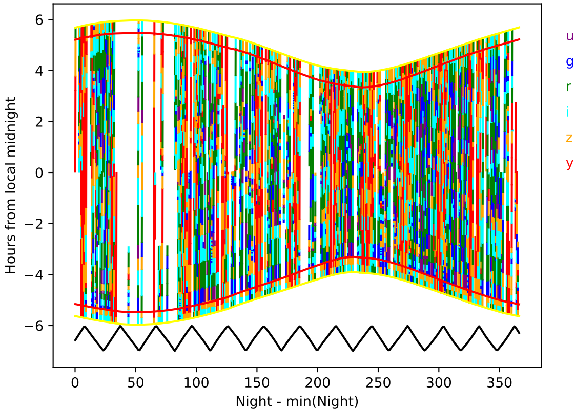
too_elab_r128_d3_giz_v3.4_10yrs year 3-4: Hourglass
