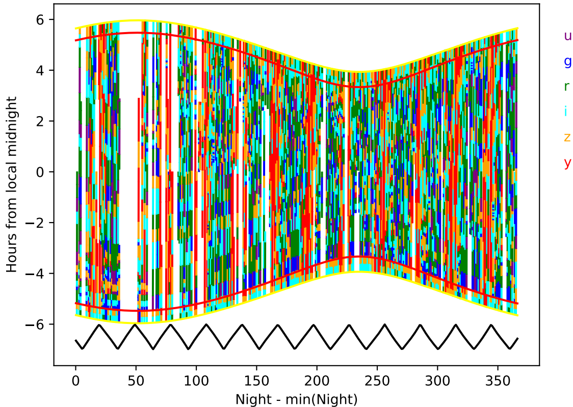
too_elab_r128_d3_giz_v3.4_10yrs year 2-3: Hourglass
