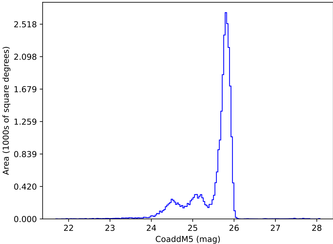
too_elab_r128_d3_giz_v3.4_10yrs z: CoaddM5
