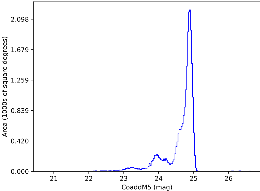
too_elab_r128_d3_giz_v3.4_10yrs y: CoaddM5
