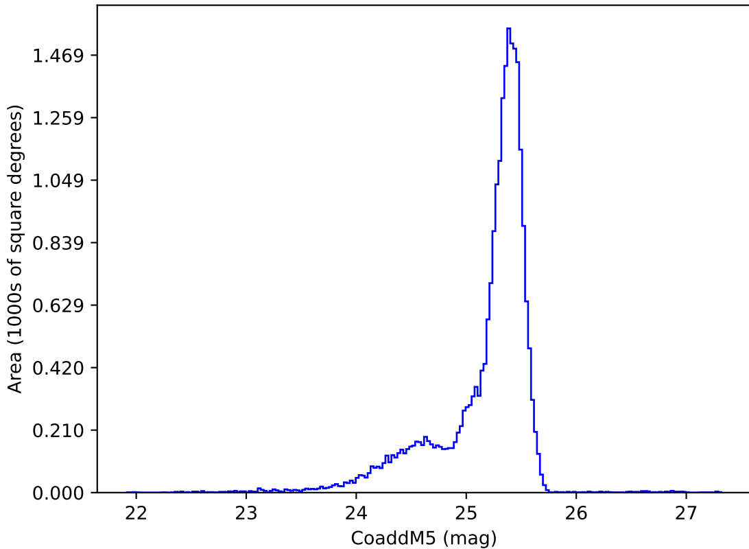
too_elab_r128_d3_giz_v3.4_10yrs u: CoaddM5
