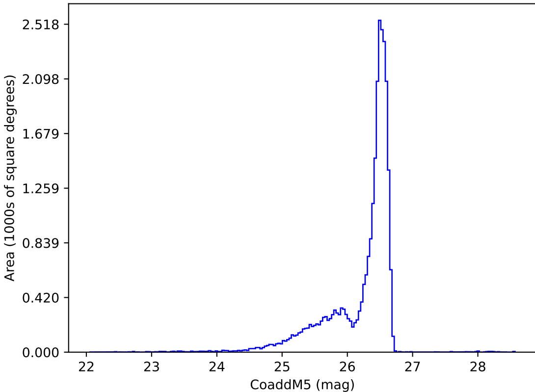
too_elab_r128_d3_giz_v3.4_10yrs i: CoaddM5
