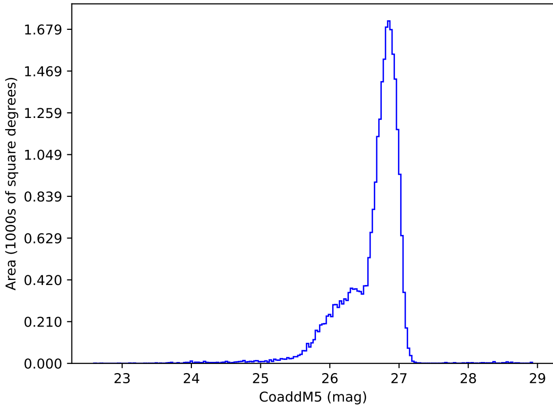
too_elab_r128_d3_giz_v3.4_10yrs g: CoaddM5
