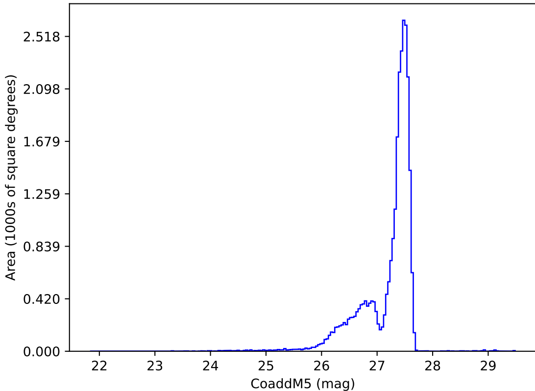
too_elab_r128_d3_giz_v3.4_10yrs : CoaddM5
