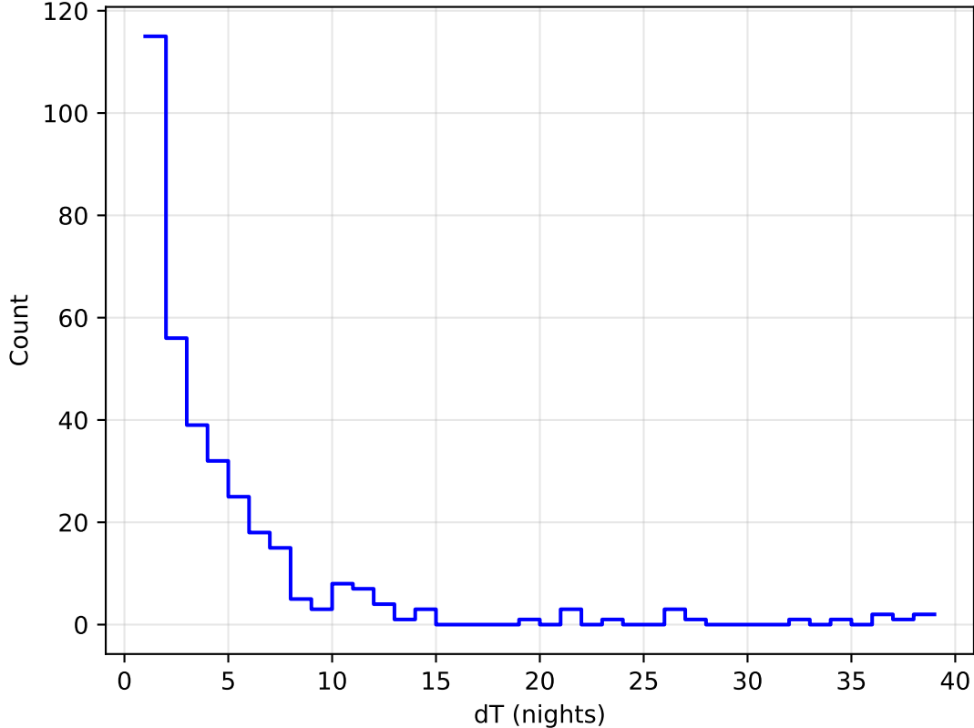
too_elab_r128_d3_giz_v3.4_10yrs all bands: DD:WFD Delta Nights Histogram
