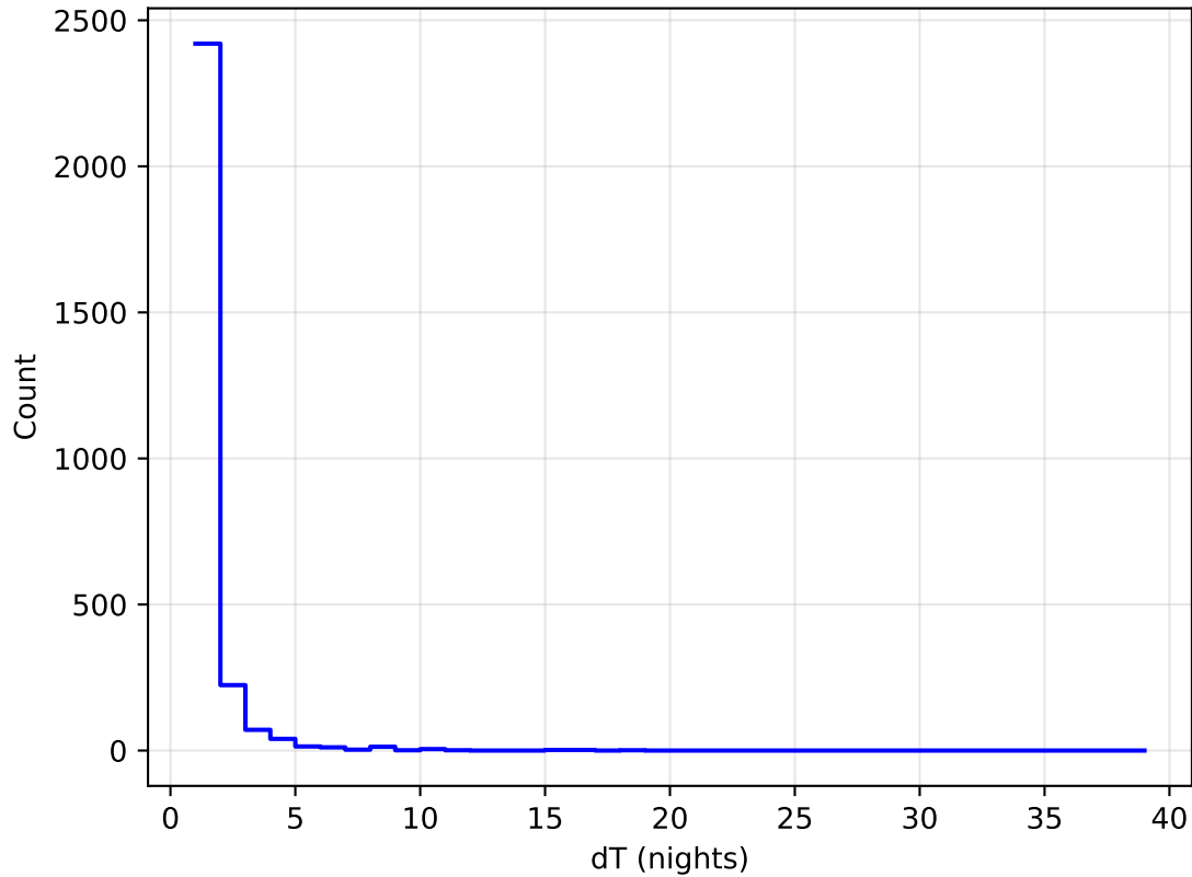
too_elab_r128_d3_giz_v3.4_10yrs all bands: DD:WFD Delta Nights Histogram
