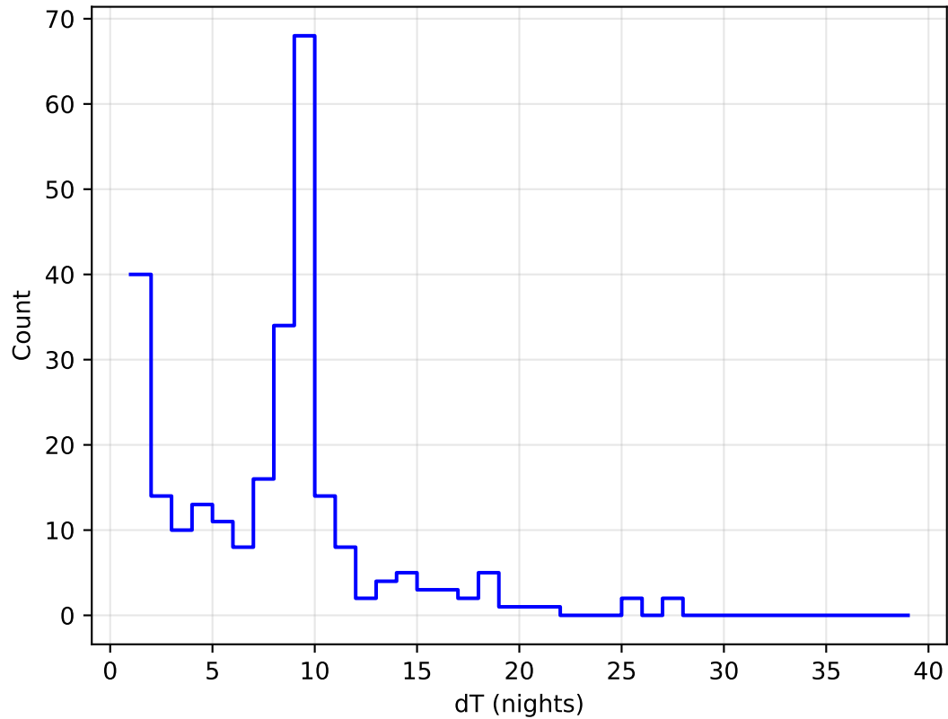
too_elab_r128_d3_giz_v3.4_10yrs all bands: DD:ELAISS1 Delta Nights Histogram
