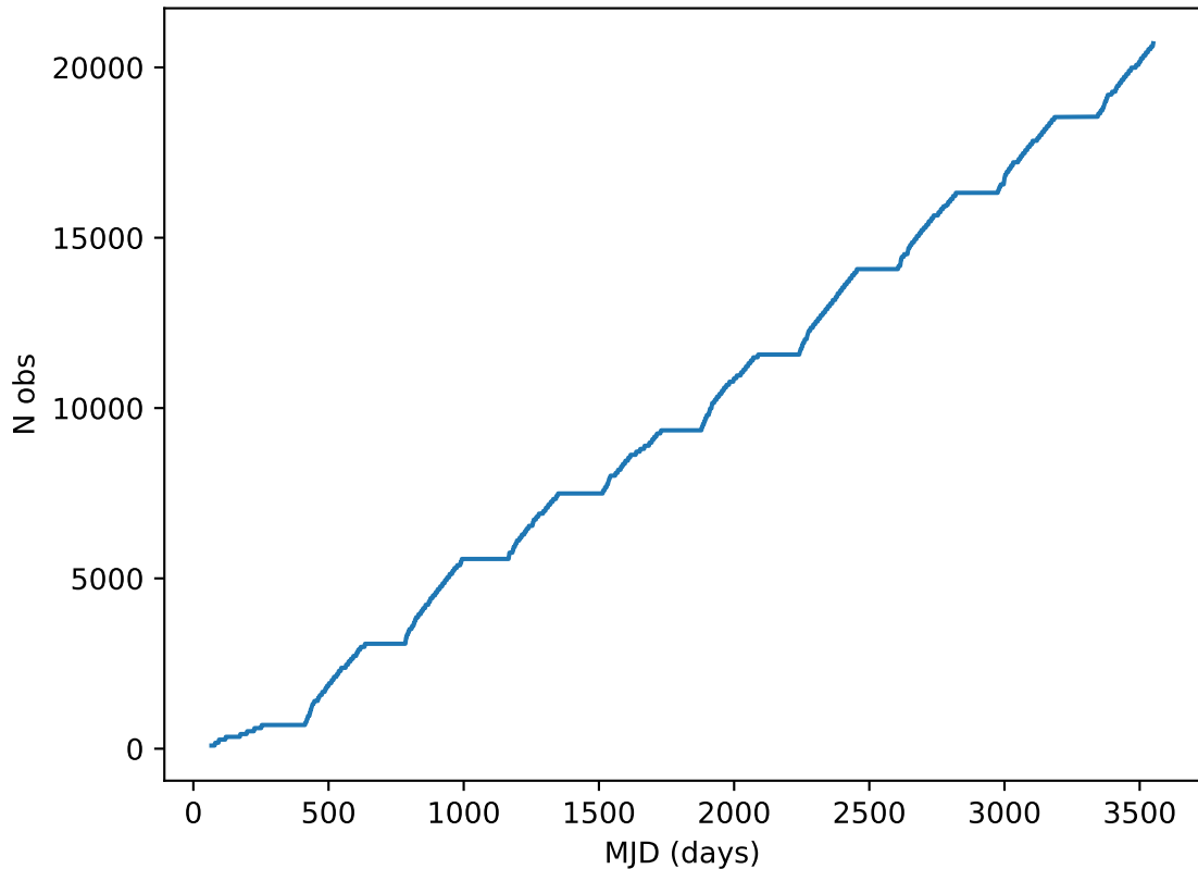
too_elab_r128_d3_giz_v3.4_10yrs all bands: DD:ELAISS1 Cumulative NVisits
