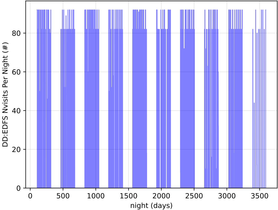
too_elab_r128_d3_giz_v3.4_10yrs all bands: DD:EDFS Nvisits Per Night
