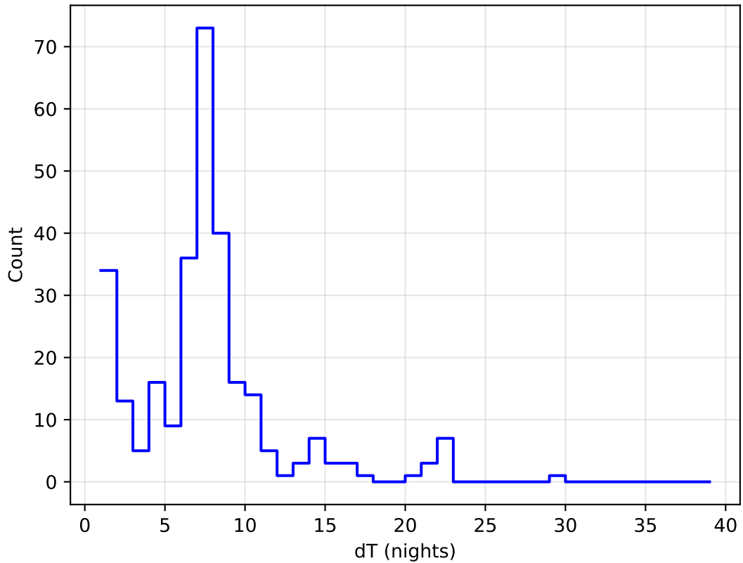
too_elab_r128_d3_giz_v3.4_10yrs all bands: DD:EDFS Delta Nights Histogram
