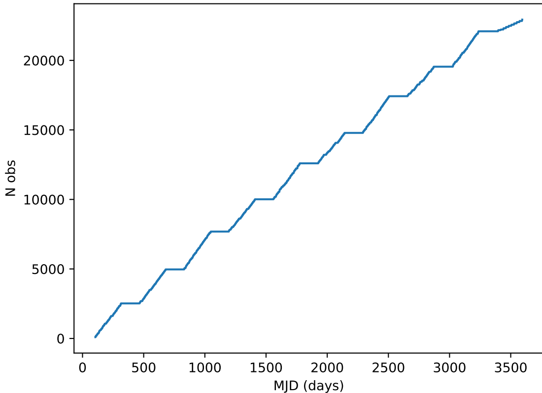
too_elab_r128_d3_giz_v3.4_10yrs all bands: DD:EDFS Cumulative NVisits
