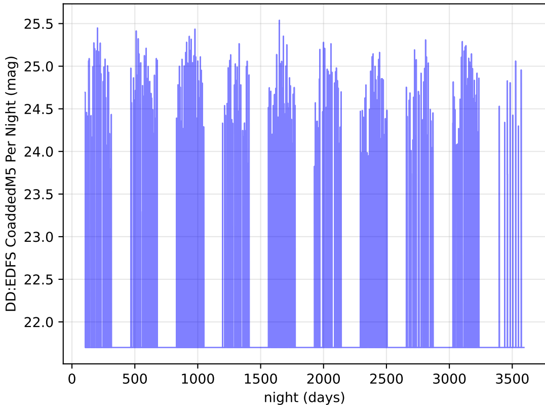
too_elab_r128_d3_giz_v3.4_10yrs z band: DD:EDFS CoaddedM5 Per Night
