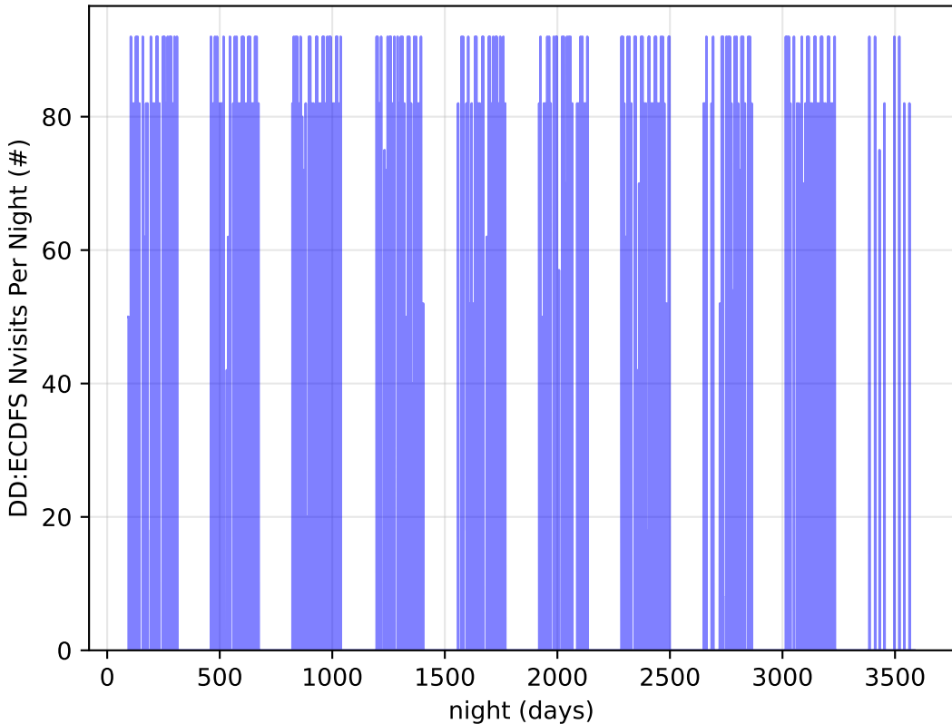
too_elab_r128_d3_giz_v3.4_10yrs all bands: DD:ECDFS Nvisits Per Night
