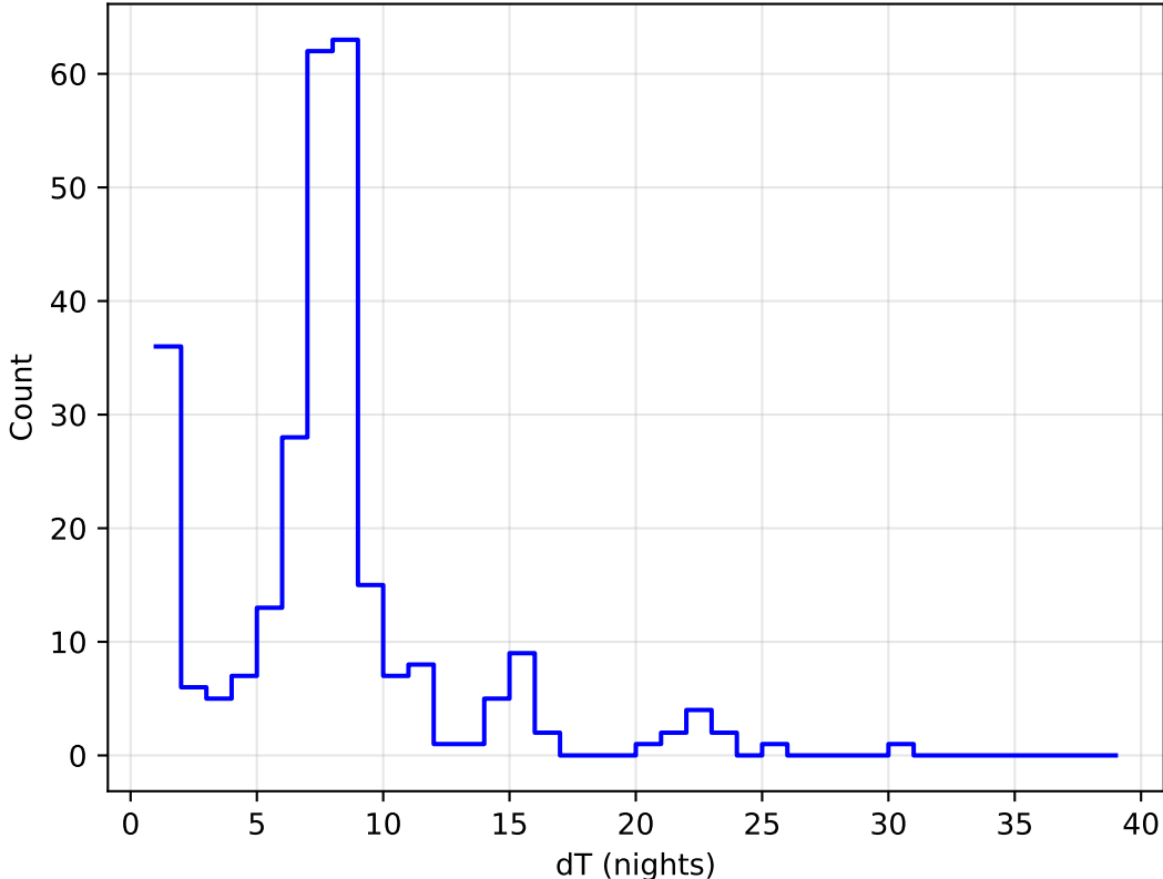
too_elab_r128_d3_giz_v3.4_10yrs all bands: DD:ECDFS Delta Nights Histogram
