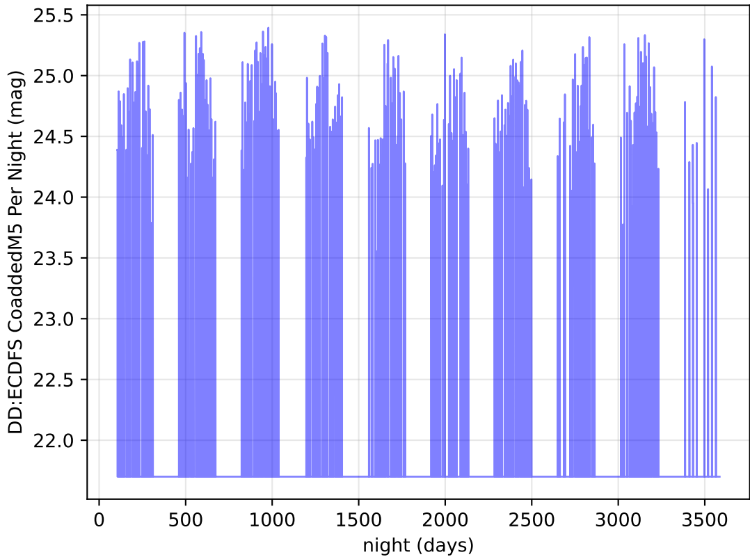
too_elab_r128_d3_giz_v3.4_10yrs z band: DD:ECDFS CoaddedM5 Per Night
