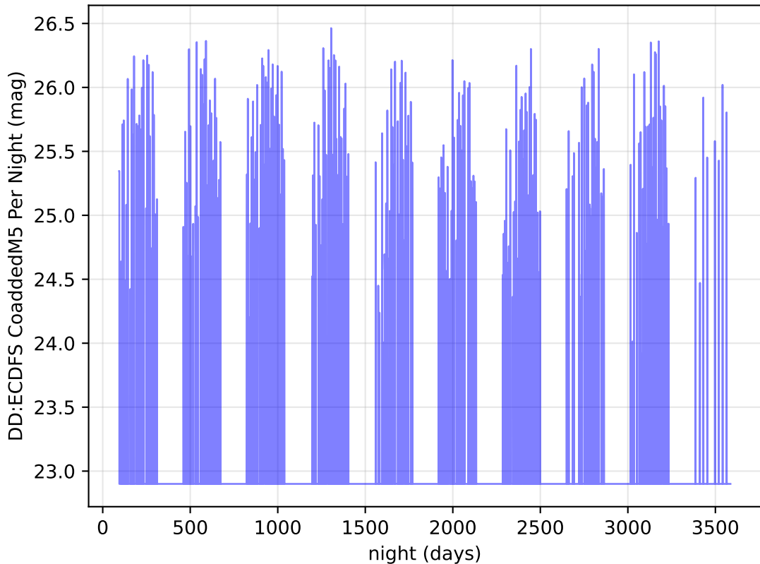
too_elab_r128_d3_giz_v3.4_10yrs r band: DD:ECDFS CoaddedM5 Per Night
