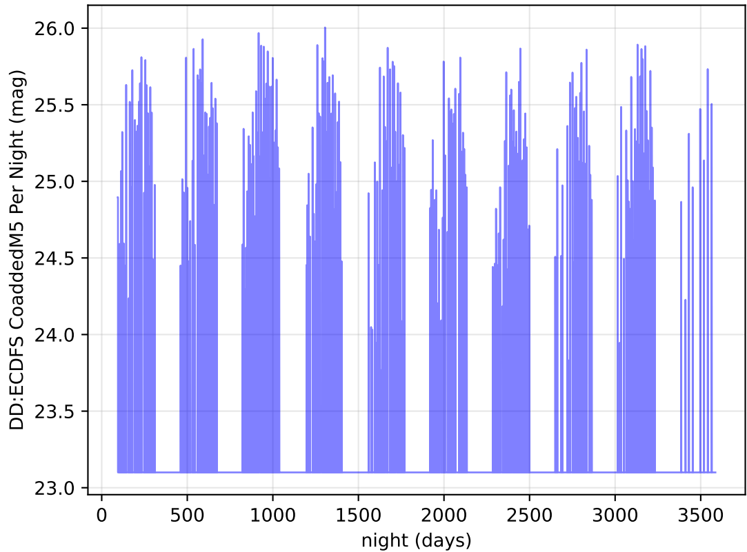
too_elab_r128_d3_giz_v3.4_10yrs i band: DD:ECDFS CoaddedM5 Per Night
