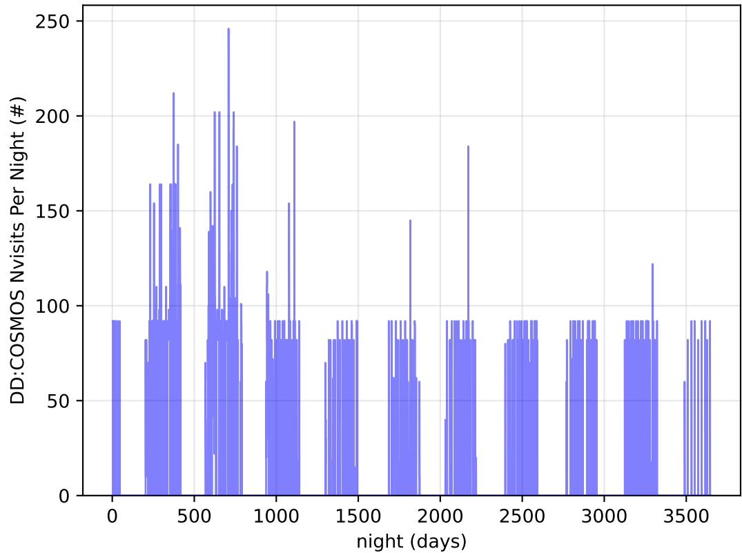
too_elab_r128_d3_giz_v3.4_10yrs all bands: DD: COSMOS Nvisits Per Night
