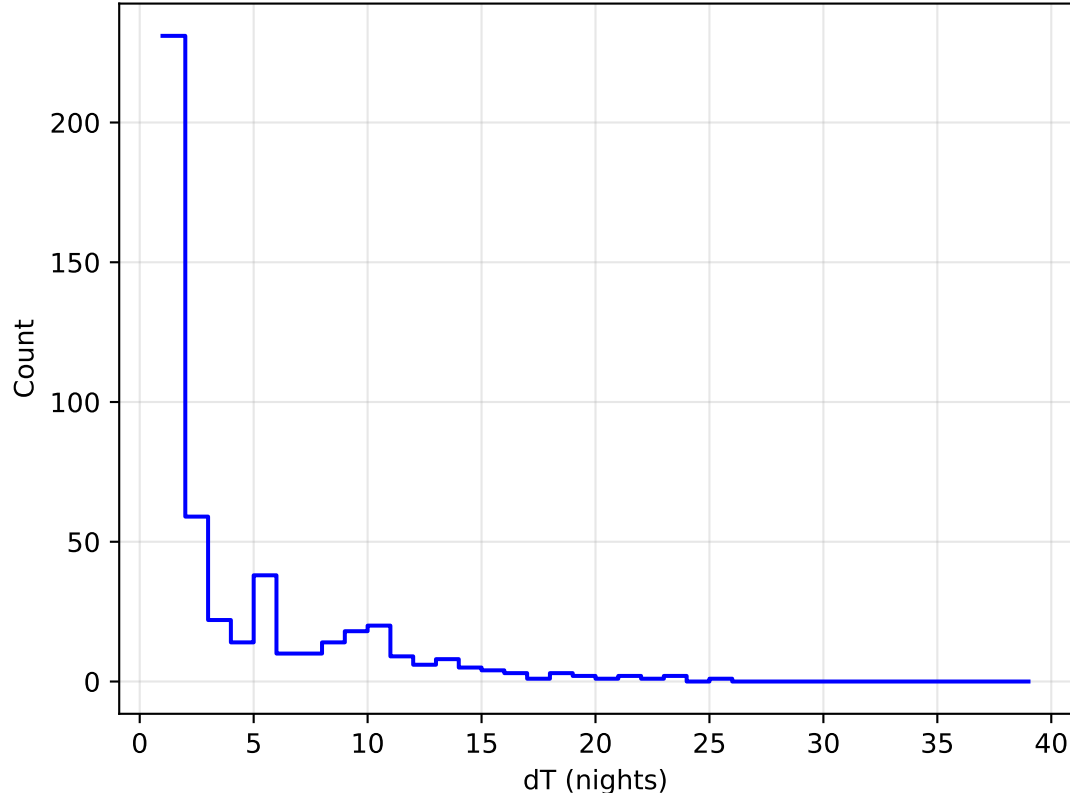
too_elab_r128_d3_giz_v3.4_10yrs all bands: DD: COSMOS Delta Nights Histogram
