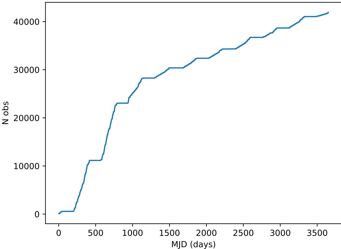
too_elab_r128_d3_giz_v3.4_10yrs all bands: DD: COSMOS Cumulative NVisits
