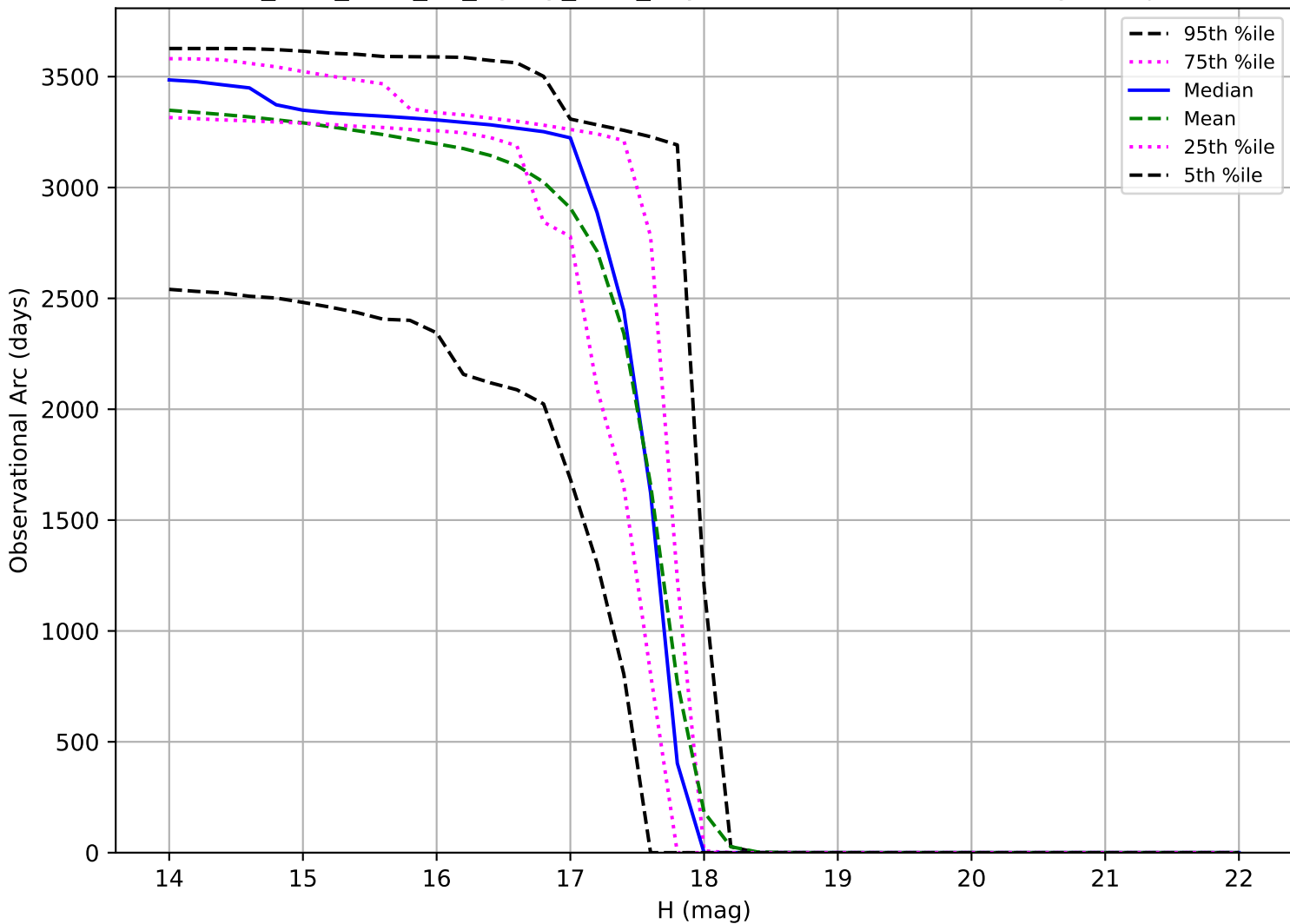
too_elab_r128_d2_ugrizy_v3.4_10yrs: Observational Arc Length Trojan
