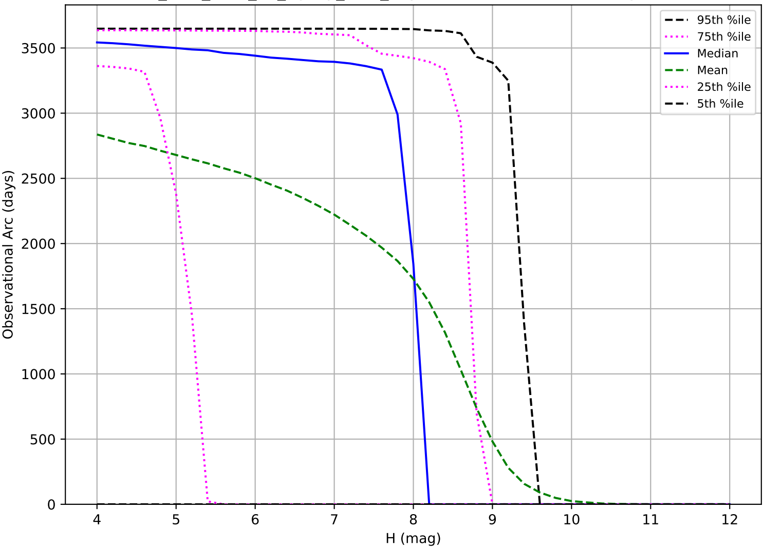
too_elab_r128_d2_ugrizy_v3.4_10yrs: Observational Arc Length TNO
