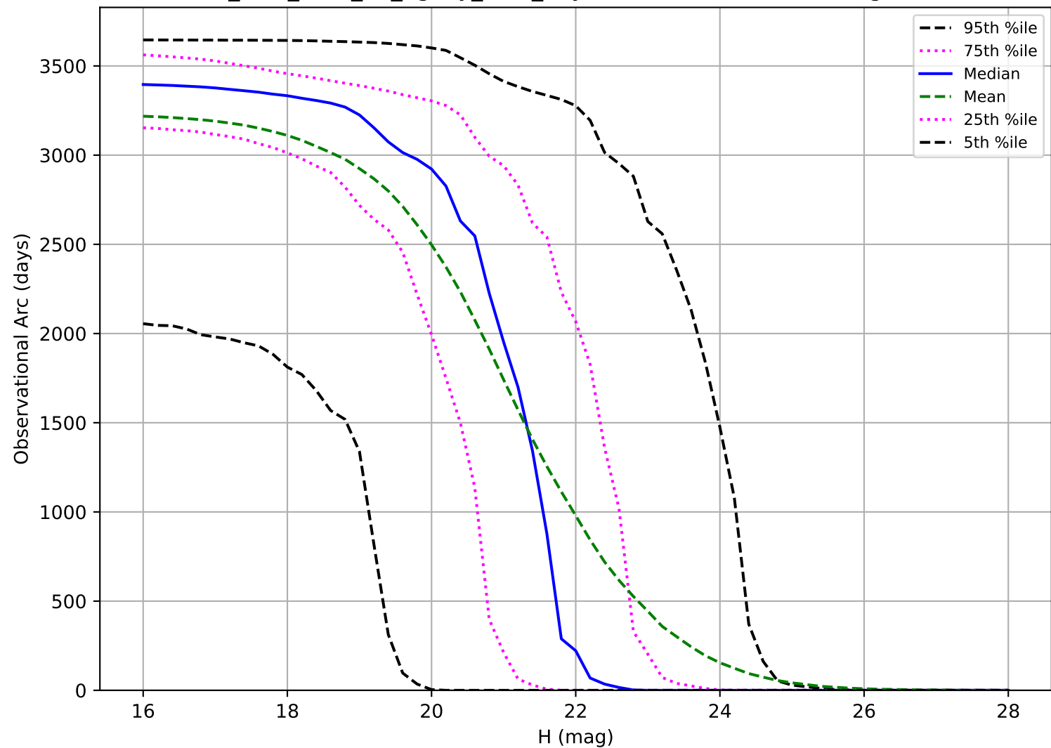
too_elab_r128_d2_ugrizy_v3.4_10yrs: Observational Arc Length PHA
