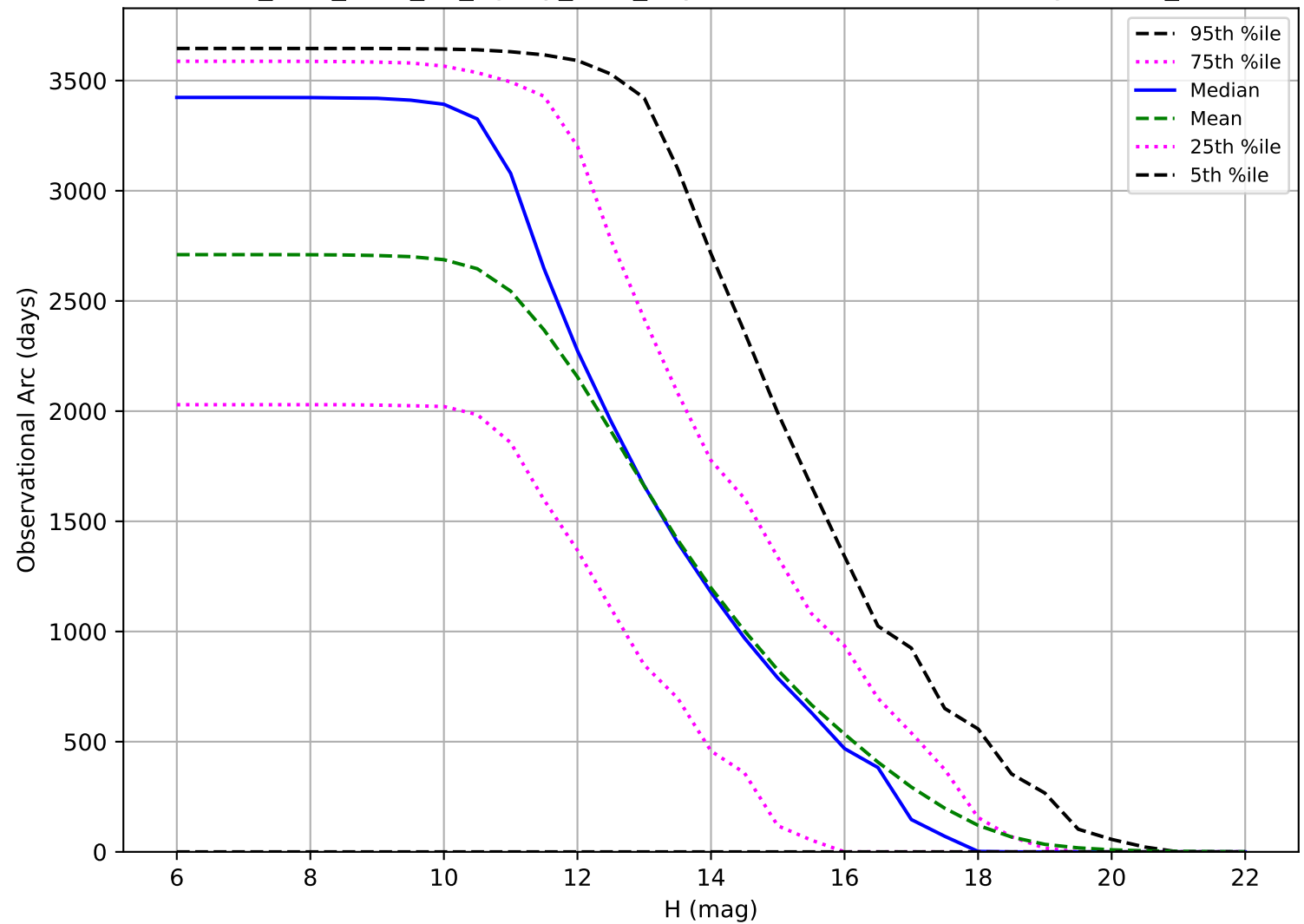
too_elab_r128_d2_ugrizy_v3.4_10yrs: Observational Arc Length OCC_r5
