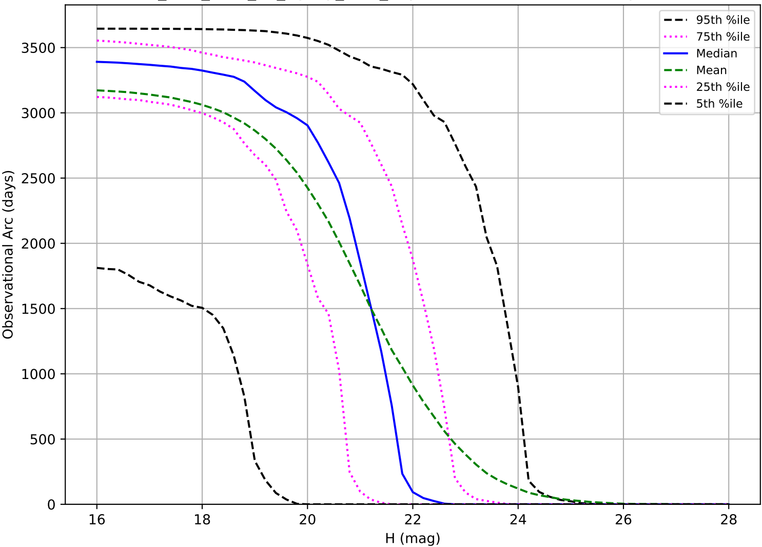
too_elab_r128_d2_ugrizy_v3.4_10yrs: Observational Arc Length NEO
