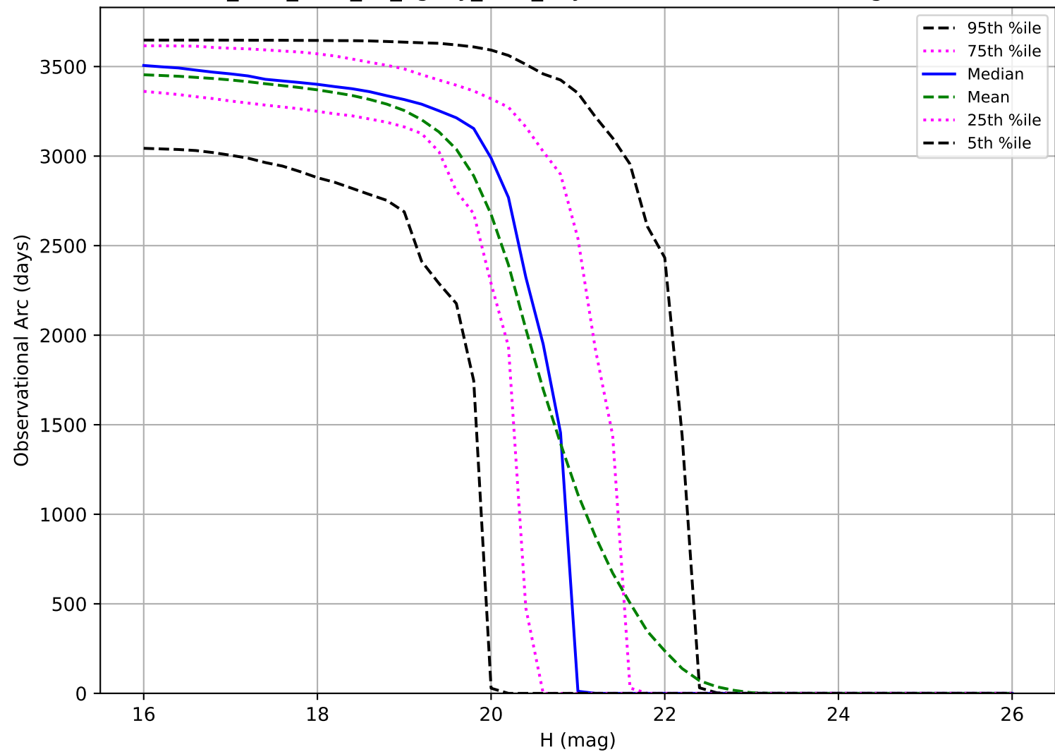
too_elab_r128_d2_ugrizy_v3.4_10yrs: Observational Arc Length MBA
