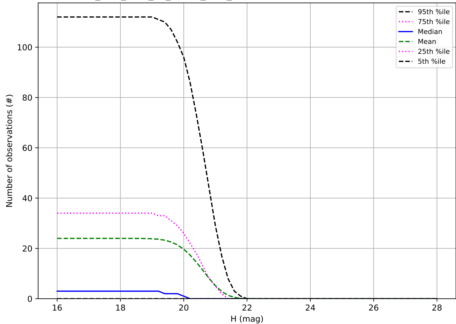
too_elab_r128_d2_ugrizy_v3.4_10yrs: Number of observations Vatira
