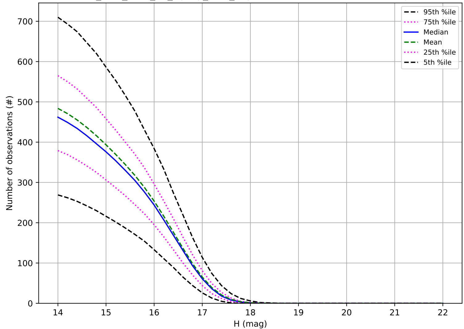
too_elab_r128_d2_ugrizy_v3.4_10yrs: Number of observations Trojan
