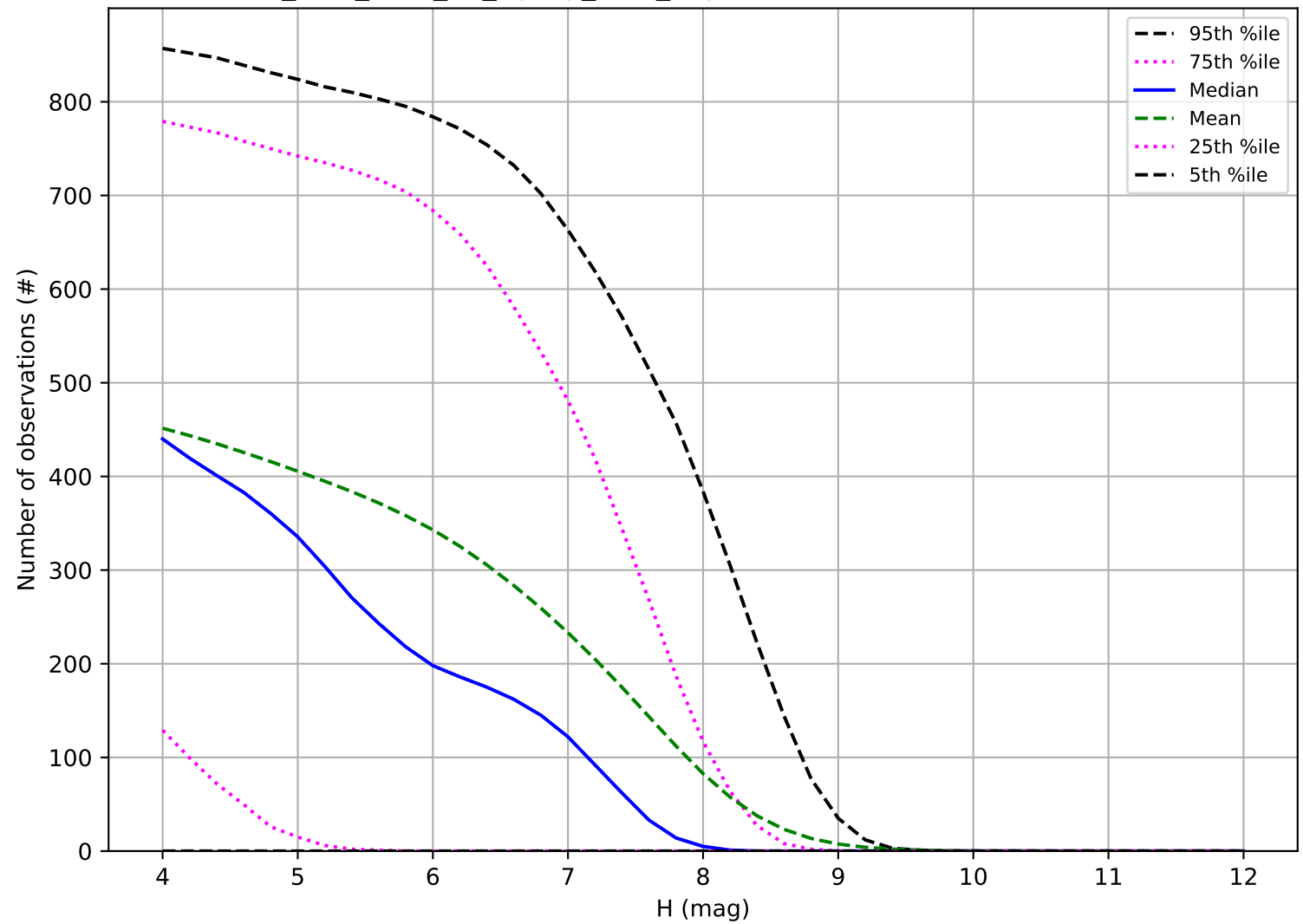
too_elab_r128_d2_ugrizy_v3.4_10yrs: Number of observations TNO
