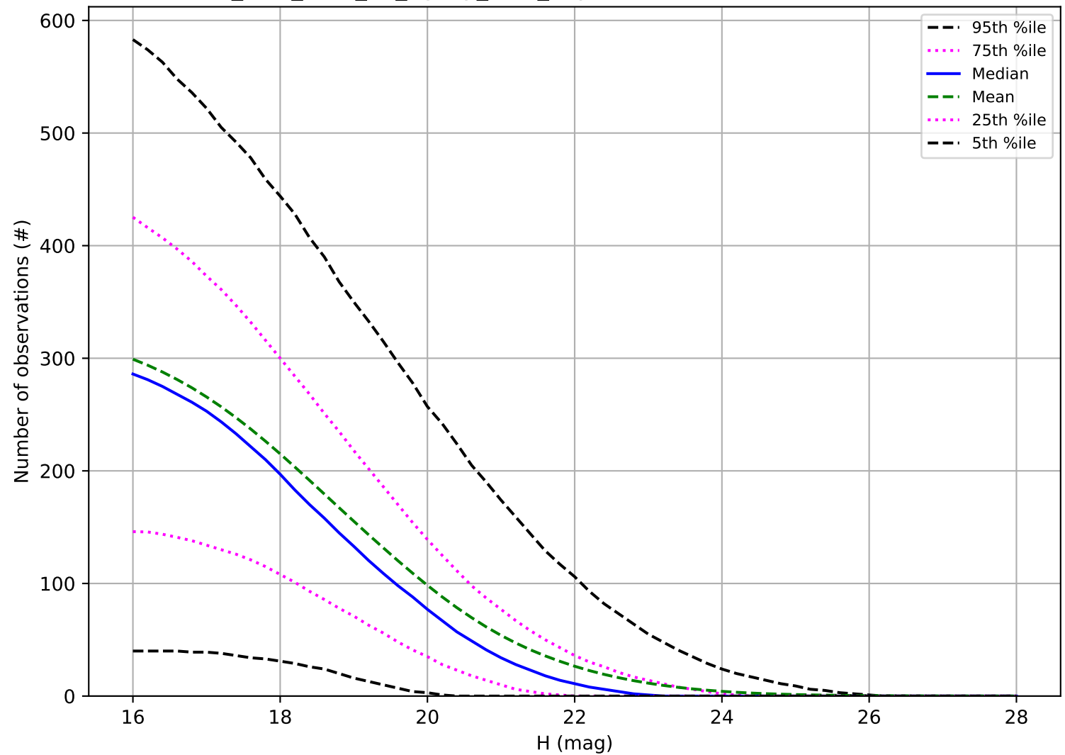
too_elab_r128_d2_ugrizy_v3.4_10yrs: Number of observations PHA
