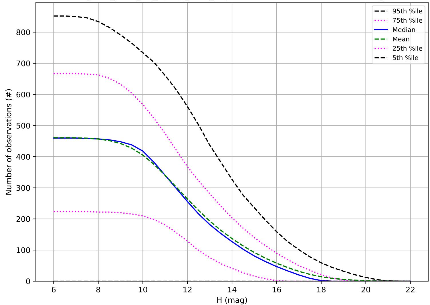
too_elab_r128_d2_ugrizy_v3.4_10yrs: Number of observations OCC_r5
