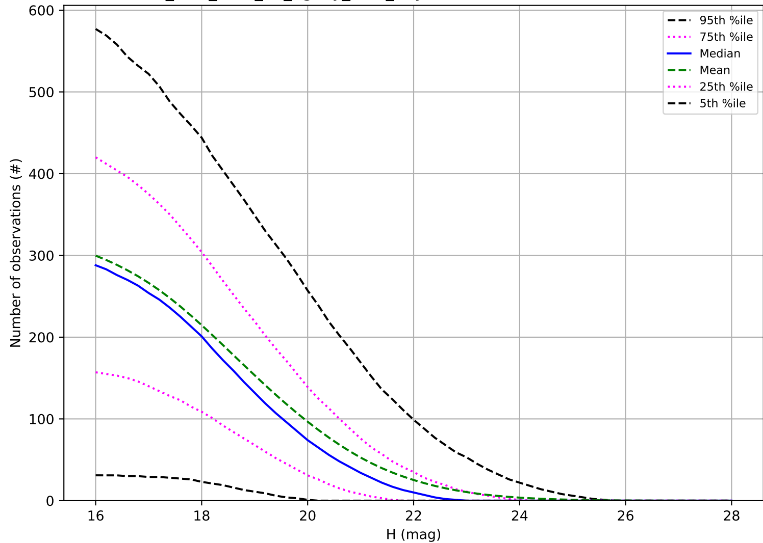
too_elab_r128_d2_ugrizy_v3.4_10yrs: Number of observations NEO
