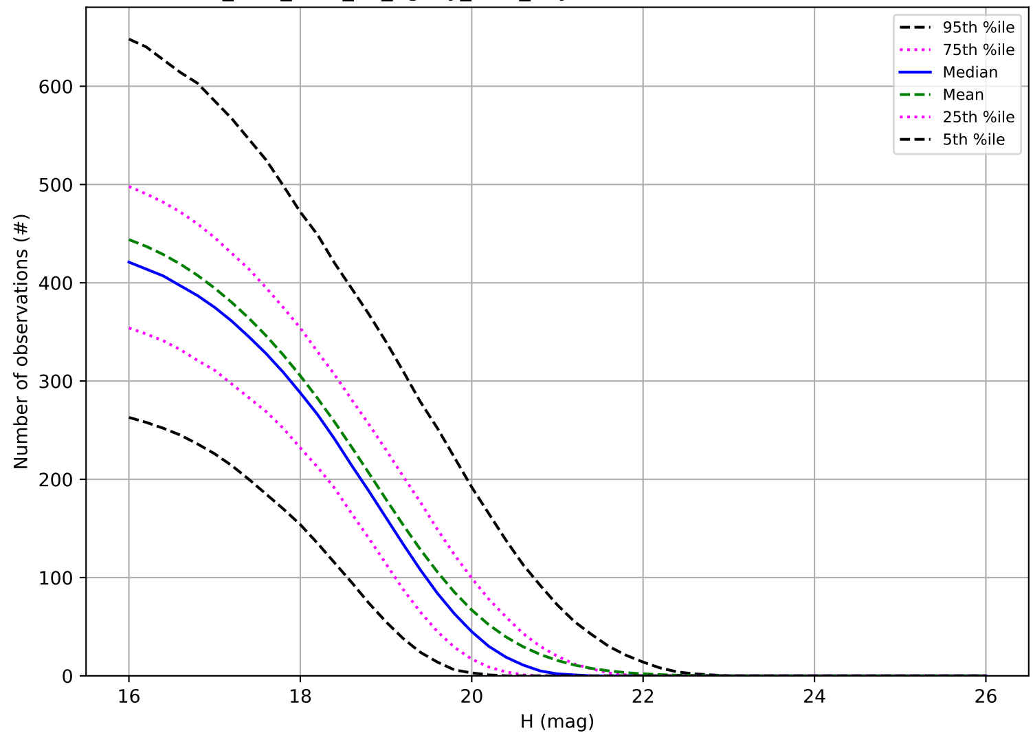
too_elab_r128_d2_ugrizy_v3.4_10yrs: Number of observations MBA
