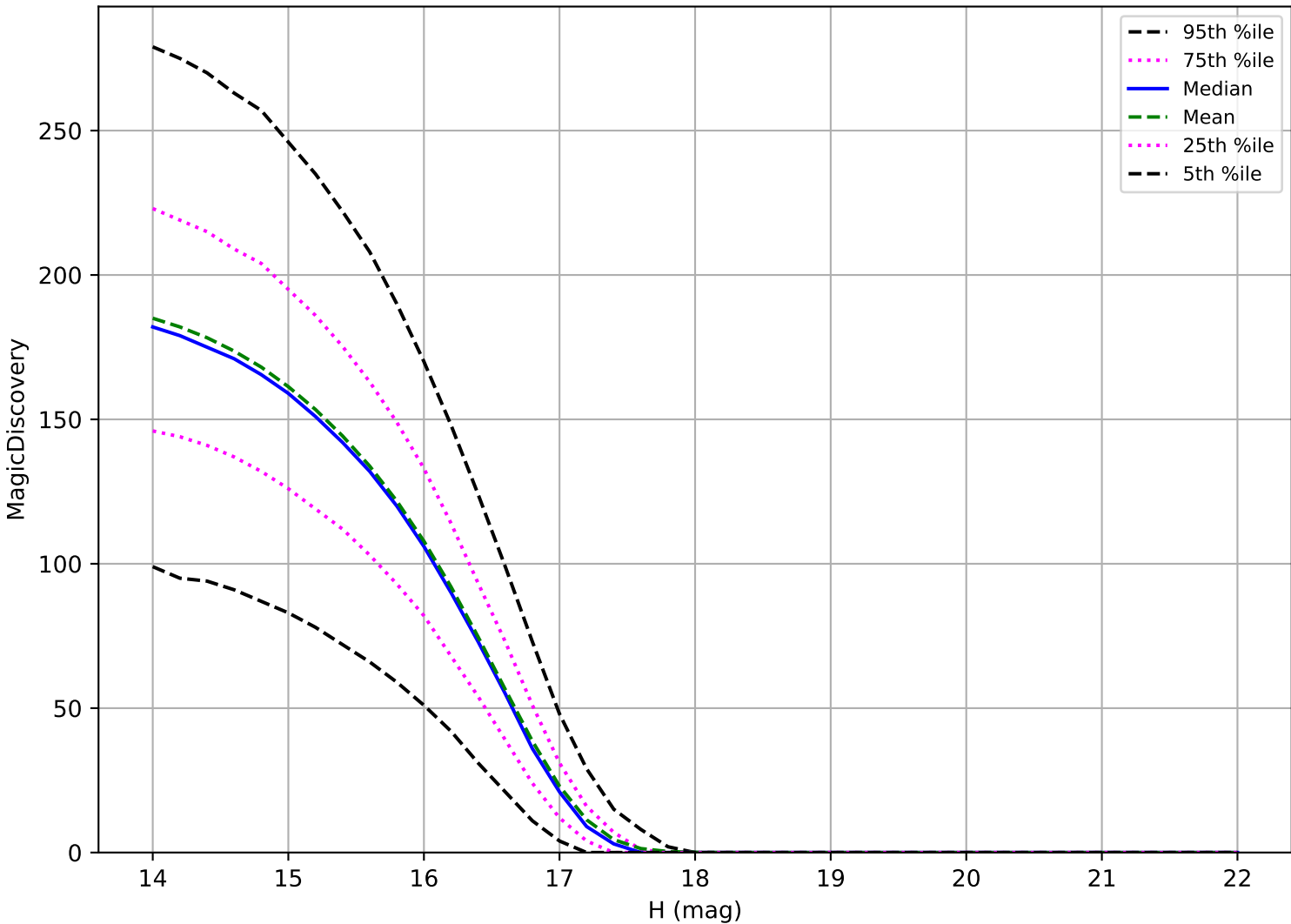
too_elab_r128_d2_ugrizy_v3.4_10yrs: Trojan 6 detections in 60 nights detection loss
